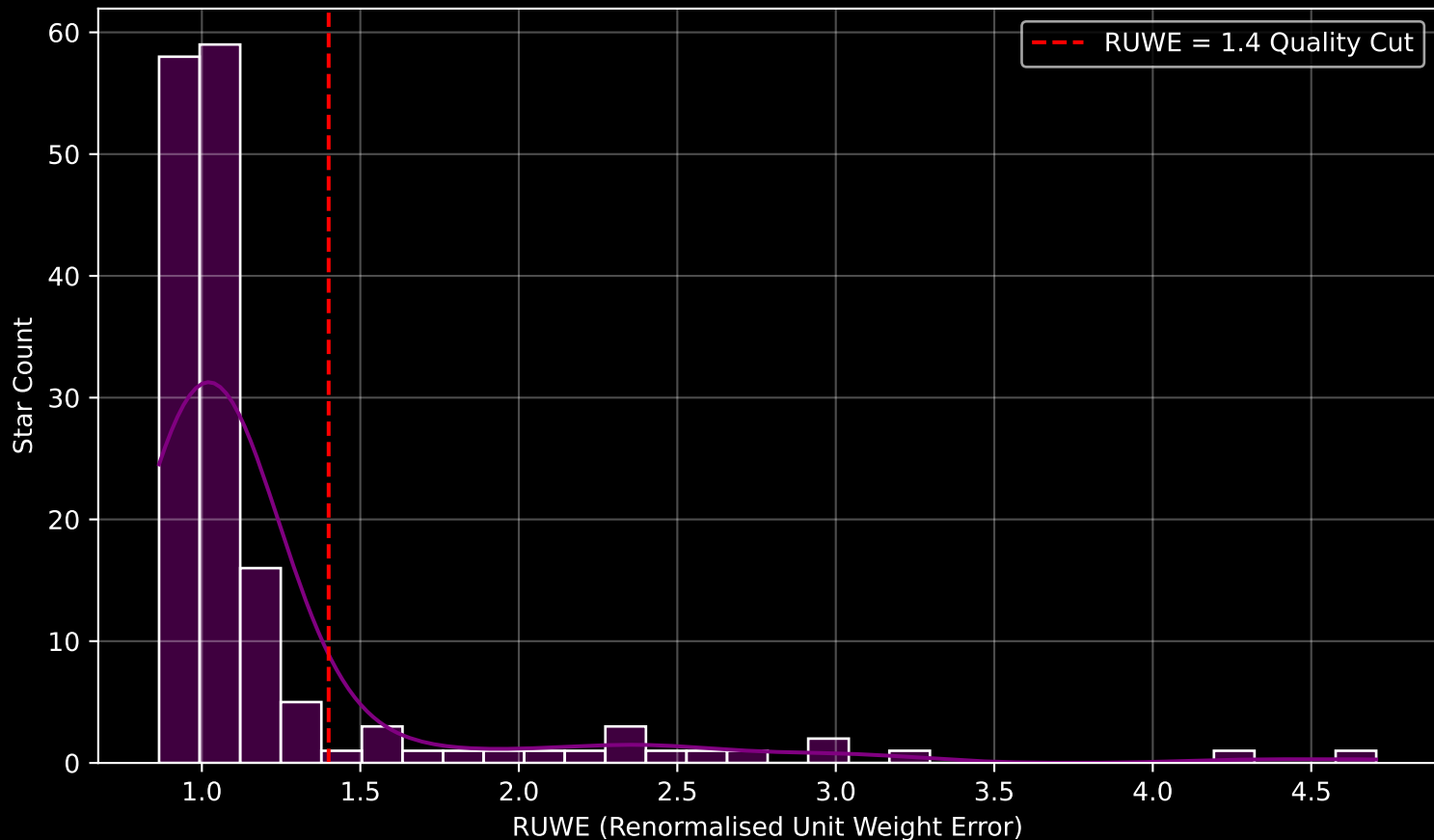
GAPOGEE DR17 Field [049+47_MGA] RUWE Distribution (n= 158)
