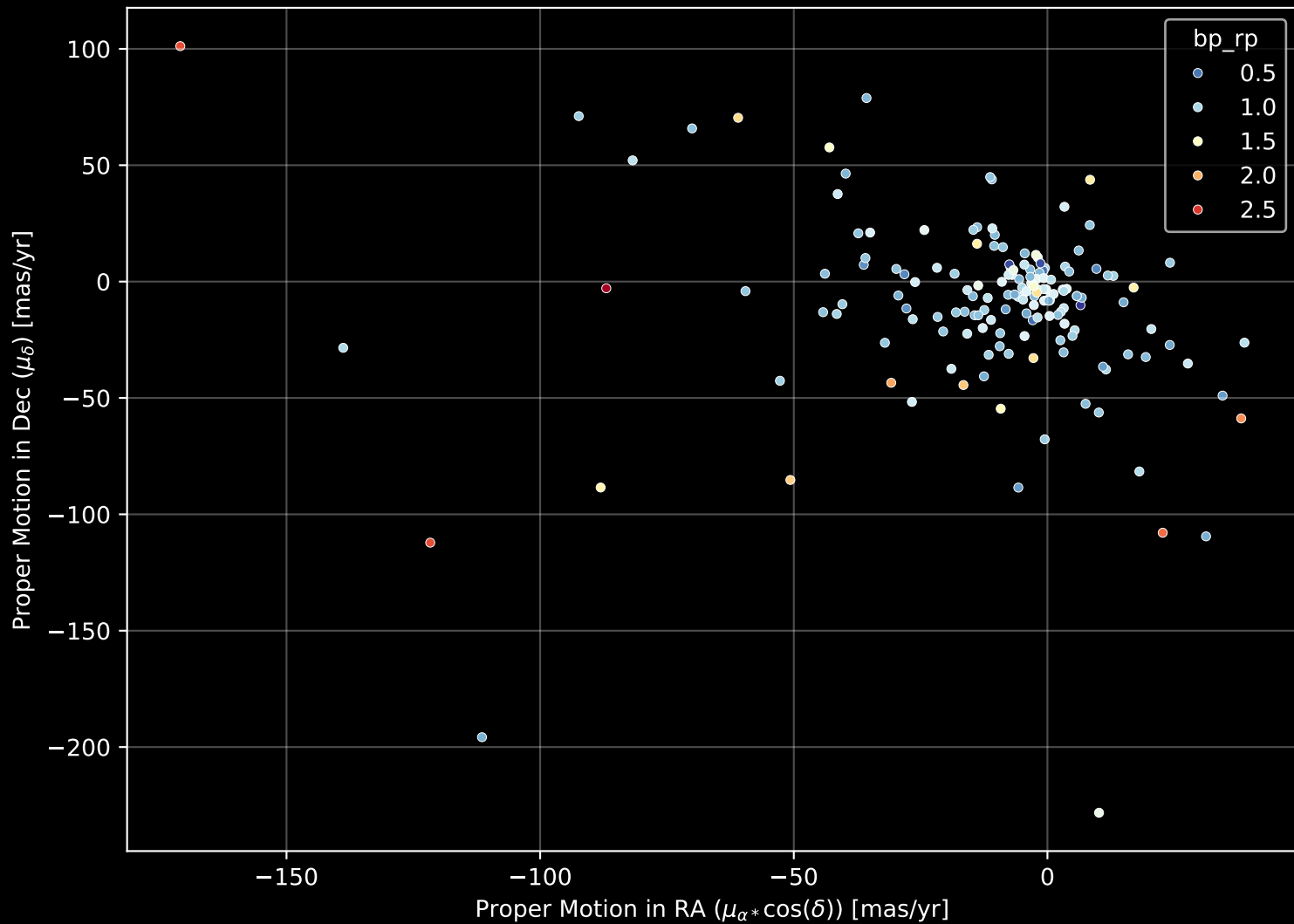
APOGEE DR17 Field: [049+47_MGA] Proper Motion Diagram (n= 161)
