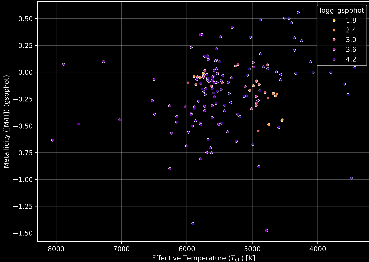
APOGEE DR17 Field: [049+47_MGA] Stellar Population Parameters (n= 161)
