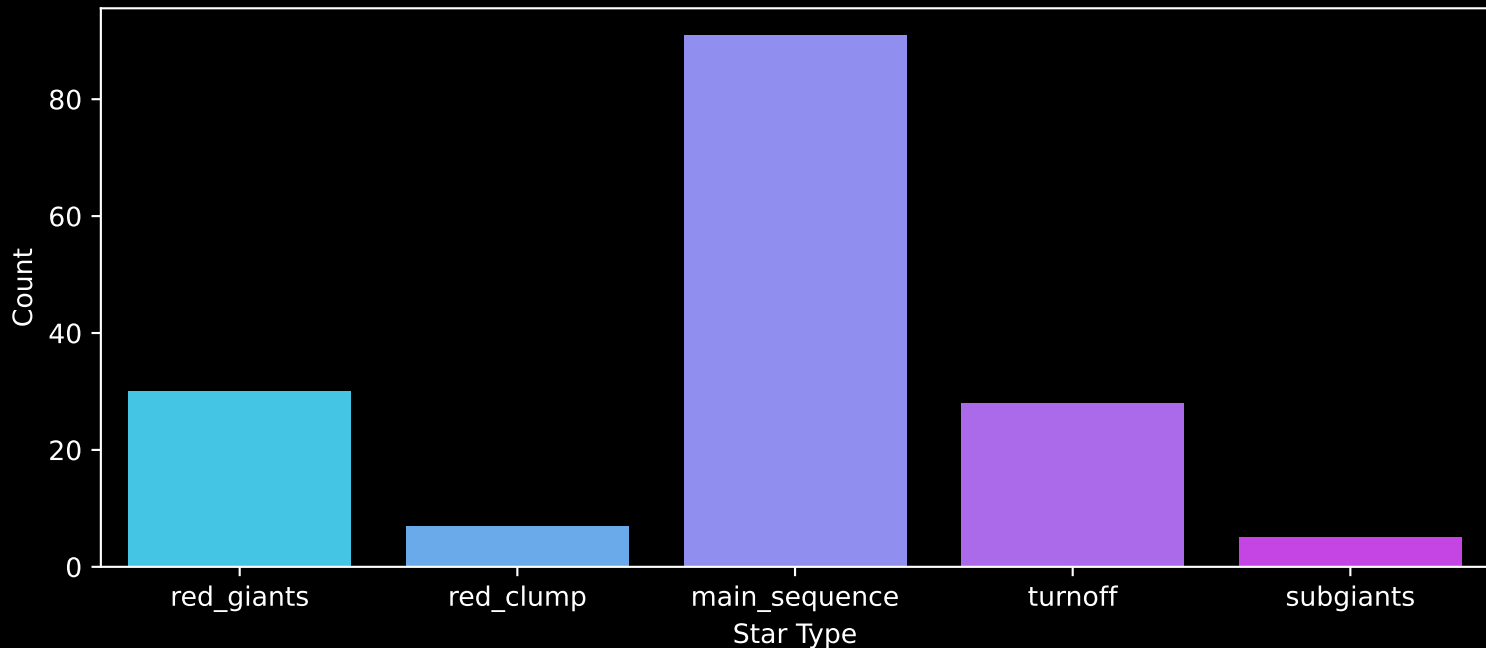
APOGEE DR17 Field: [049+47_MGA] Count plot of Star Type
