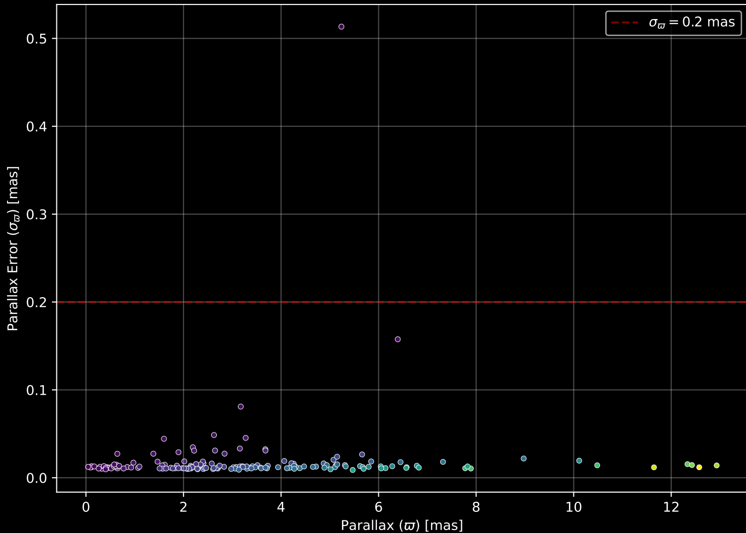
APOGEE DR17 Field: [049+47_MGA] Parallax Quality (n= 161)
